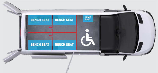
LAYOUT 6: Five compartments with side accessibility and/or high risk isolation
