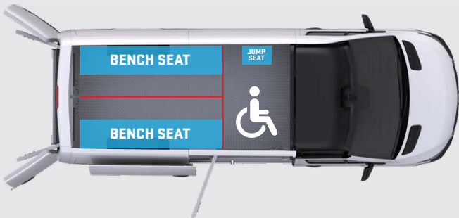
LAYOUT 5: Three compartments with side accessibility and/or high risk isolation
