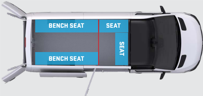
LAYOUT 3: Two compartments with short partition
