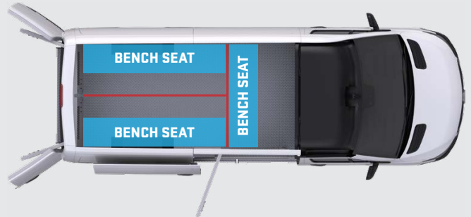
LAYOUT 4: Three compartments
